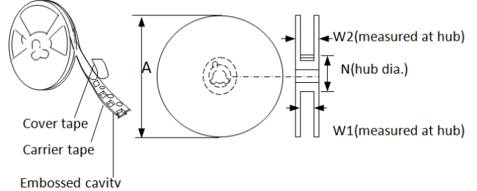
EIA Reel Dimensions
